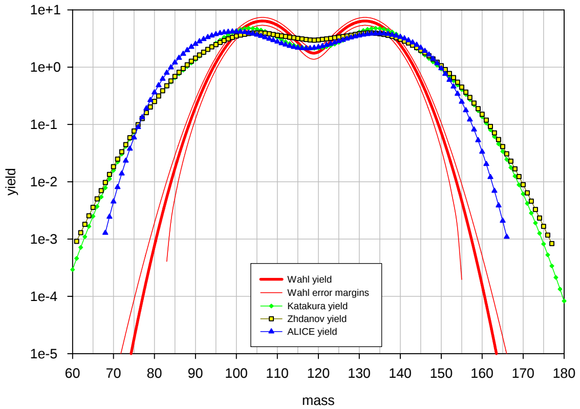
Benchmark B: ^{244}\text{Cm} at 50 MeV, post neutron emission mass distribution
